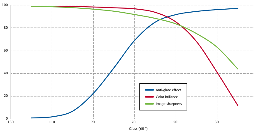
Influence of gloss on "color brilliance" and image sharpness (Source: Berliner Glas)
