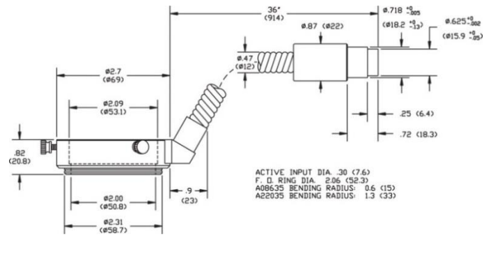
A08635 - 38 / 53 mm Ringlight with Vertical Exit
