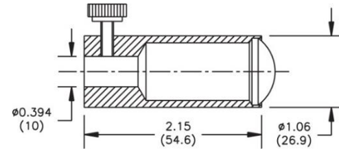
A08082 Small Spot Lens
