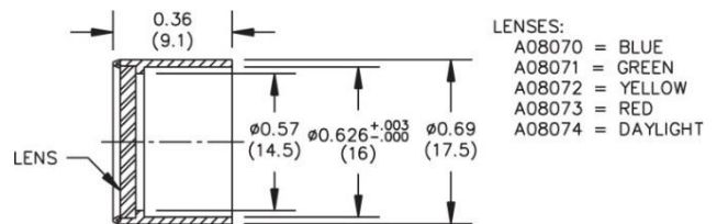
A08070 – A08074 Dichroic Color Filters
