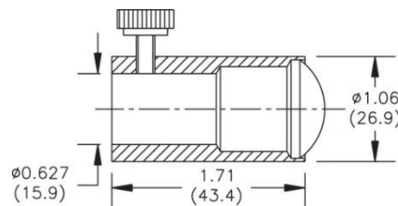
A08084 Spot Lens
