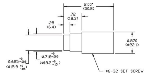
A08931 Color Filter Adapter
