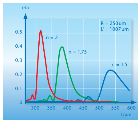
Graph of coupling efficiency vs. refractive index
