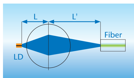
Optical sub-assembly
