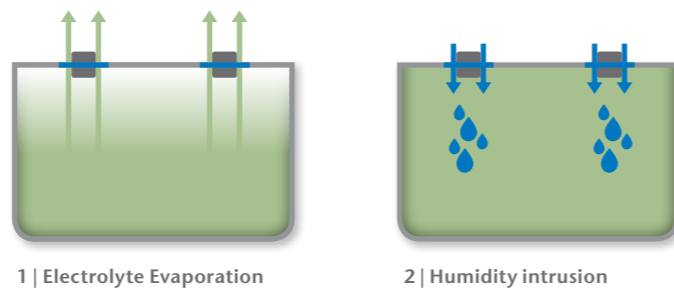
1 | Electrolyte Evaporation
