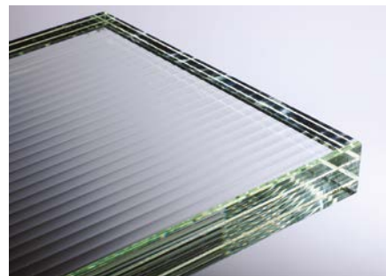
Laminated glass: 8 mm RIVULETTA® with 1.52 mm PVB foil, 10 mm floatglass, 1.52 mm PVB foil and 8 mm RIVULETTA®
