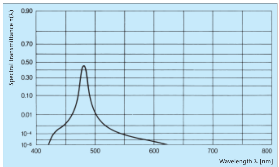
Fig. 16: Spectral transmittance curve (general curve) of filter type DMZ 12
