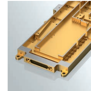
MCM housings
