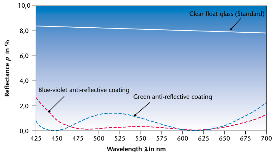
Regular spectral reflectance \rho(\lambda) of CONTURAN® of average production state
