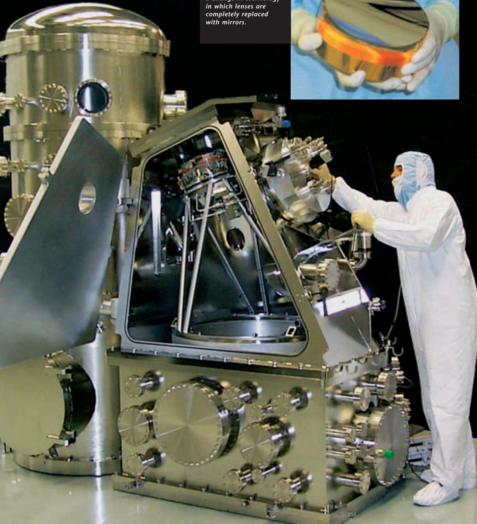
Prototype of an EUVL wafer stepper by the Lawrence Livermore National Laboratory, California, USA.
