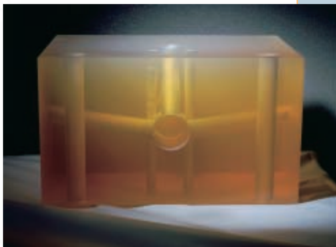
A block of “Zerodur” used for test drillings. The holes are required to house laser equipment and the ray guidance system.
