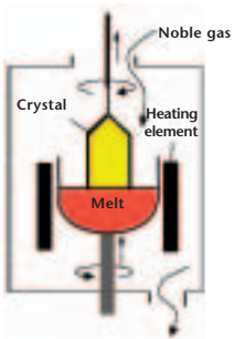
Schematic view of the Czochralski (Cz) method.
