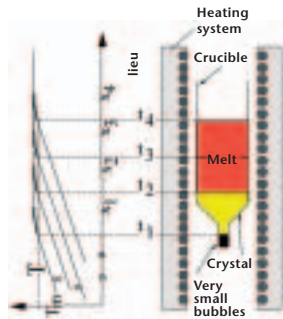
Sketch of the furnace temperature profile for various time stages in a Vertical Gradient Freeze (VGF) configuration.
