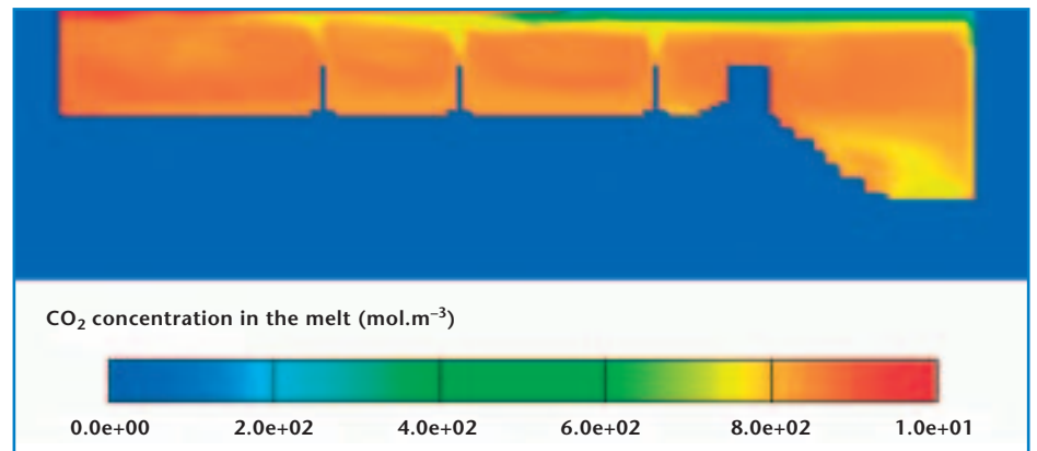
Calculated distribution of dissolved CO 2 in a melting tank (concentration contours in the vertical cross-section of a melting tank.)
