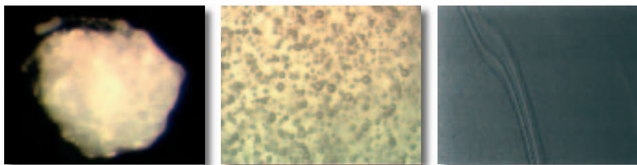
Batch stones (unmelted batch), bubble seeds and cords. Some typical imperfections in glass, caused by incomplete melting, incomplete fining and insufficient homogenization (from left to right).
