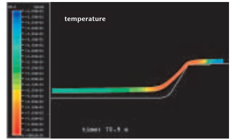
An accurately timed and geometrically accurate simulation of rapid hot forming can be achieved with the aid of a good approximation for the heat transport by radiation.
