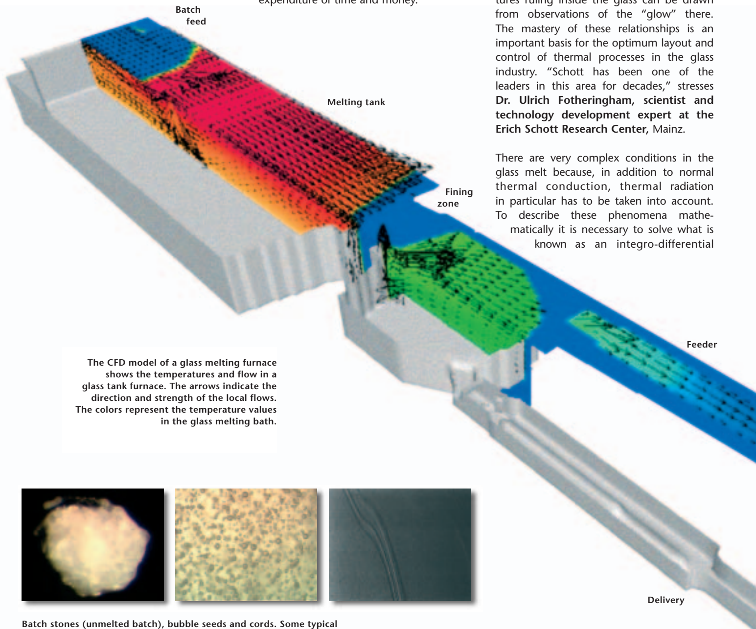
Batch stones (unmelted batch), bubble seeds and cords. Some typical imperfections in glass, caused by incomplete melting, incomplete fining and insufficient homogenization (from left to right).
