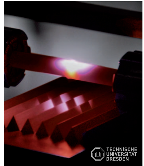
Sealing of the technical ceramic can be achieved through a conventional temperature program in a furnace or through laser welding.
