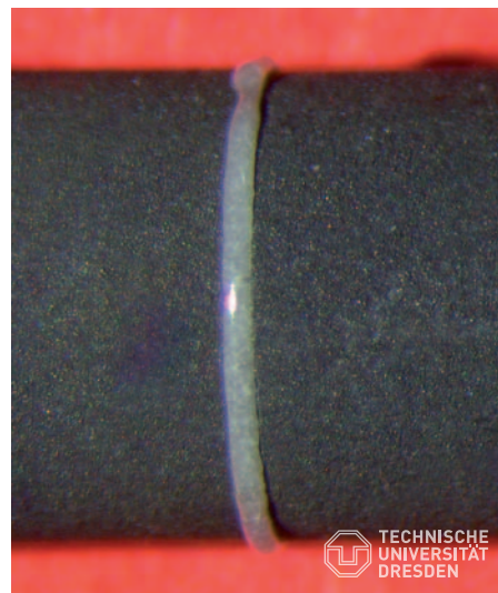
Joining of SiC ceramic with SCHOTT sealing glass.
