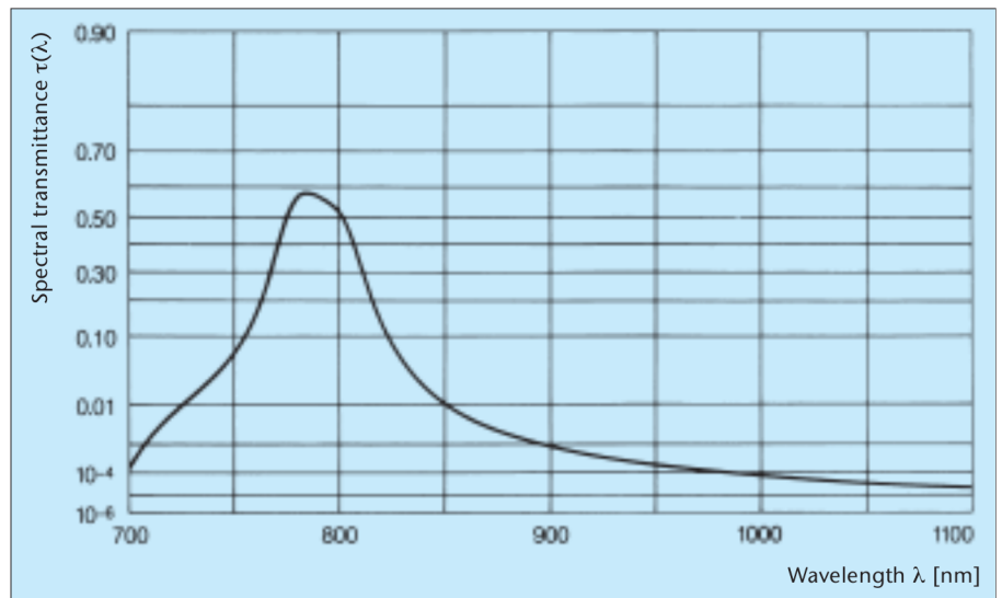
Fig. 20: Spectral transmittance curve (general curve) of filter type KMZ 50
