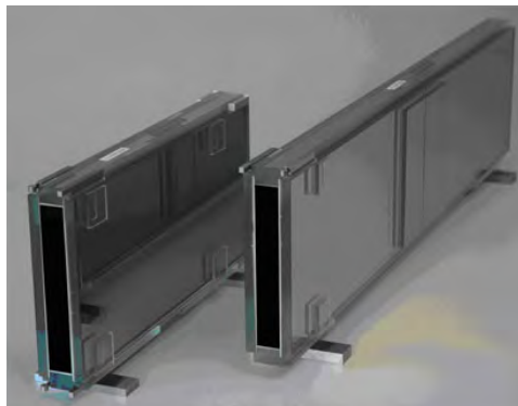
Fig. 1: Neutron guide fabricated by SwissNeutronics for the Institute Laue-Langevin in Grenoble. The glass plates are coated with supermirror m = 2 .
