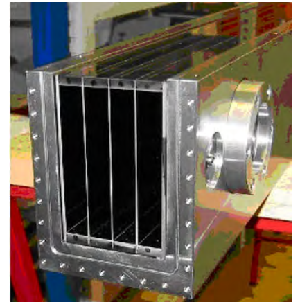
Fig. 3: Multi-channel neutron guide for the Spallation Neutron Source SNS in Oak Ridge National Laboratory (USA). The glass plates are coated with supermirror m = 3.6 . The casing is made of stainless steel.
